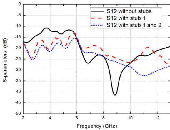
Fig. 2. Simulated S12 and S21 when total number of stubs varies.
