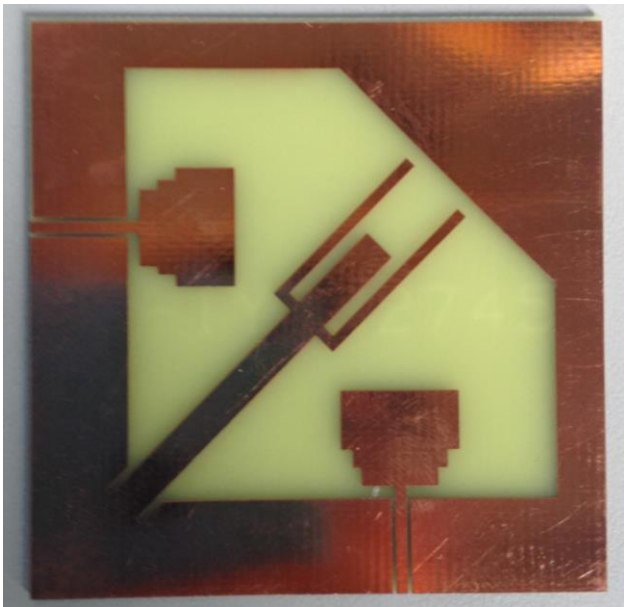
Fig. 3. Prototype of proposed antenna.
