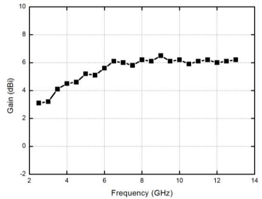
Fig. 6. Measured gain of proposed antenna.
