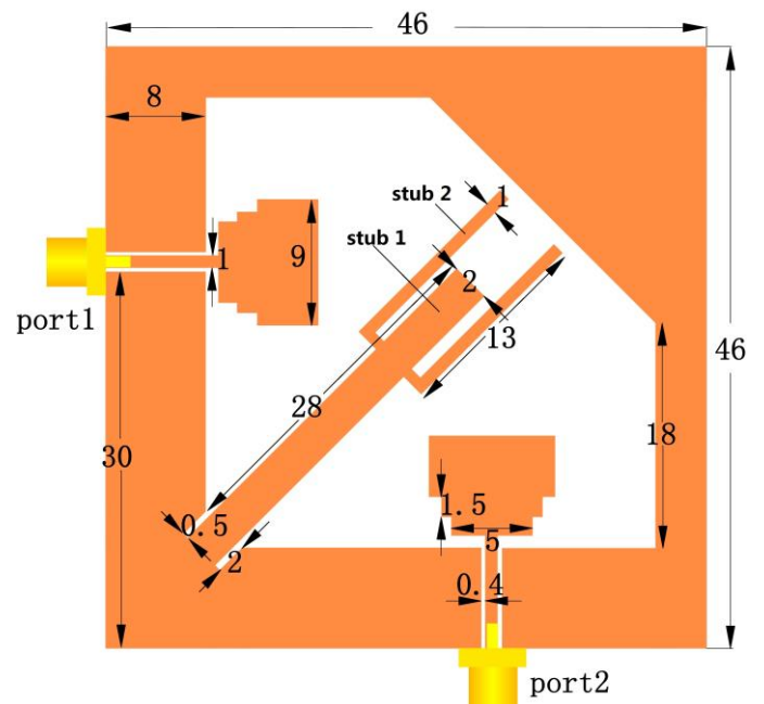
Fig. 1. Configuration and parameters of proposed antenna.
