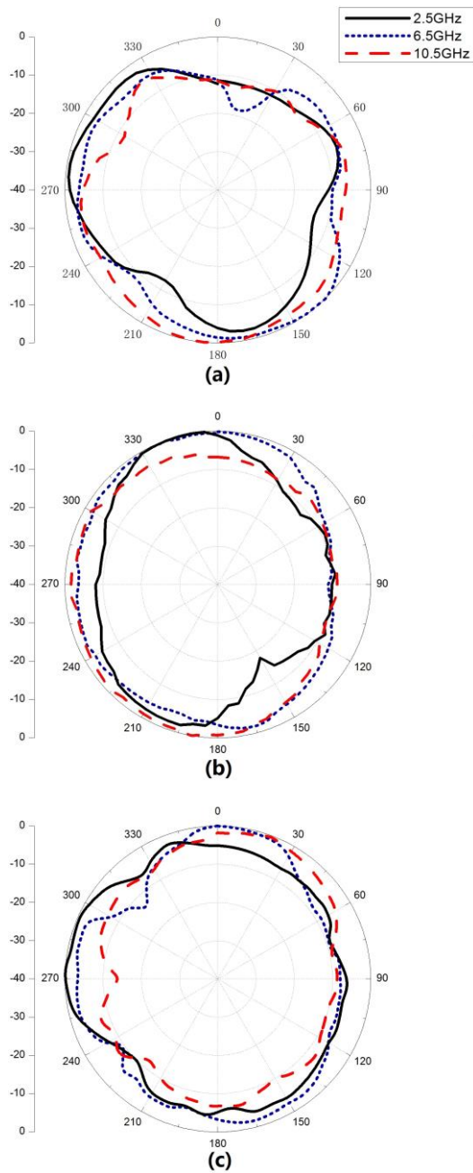
Fig. 5. Measured radiation patterns of proposed antenna at 2.5 GHz, 6.5 GHz, and 10.5 GHz: (a) XY plane, (b) XZ plane, and (c) YZ plane.
